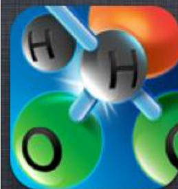
ChemIQ
